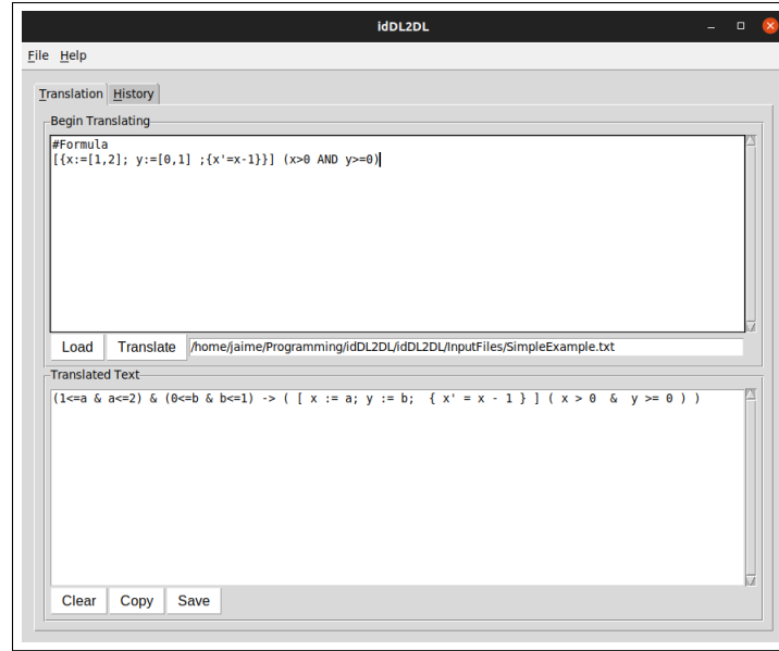
Figure 1: Translation of a simple example in idDL2dDL.
