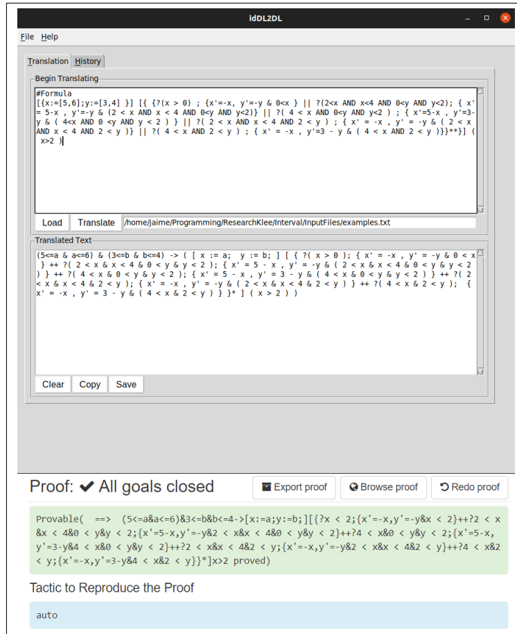
Figure 2: The translation of the biological regulatory network example in idDL2dDL and the respective proof in KeYmaera X
